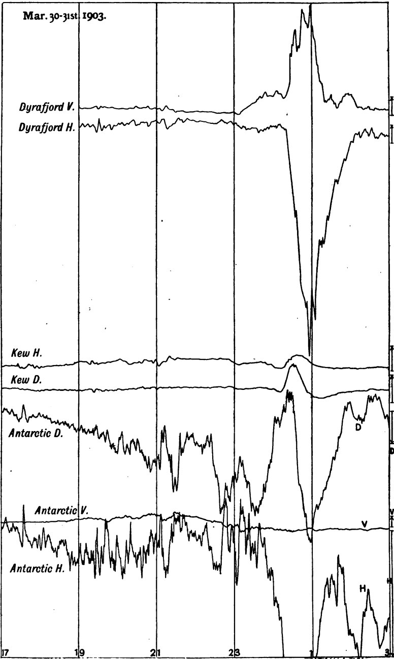
FIG. 42.—ARCTIC-KEW-ANTARCTIC CURVES,
